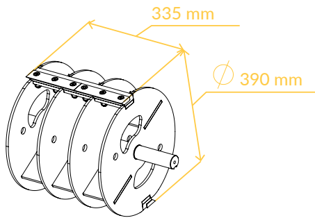
TROMMELSCHNEIDEMECHANISMUS Drum cutting system
